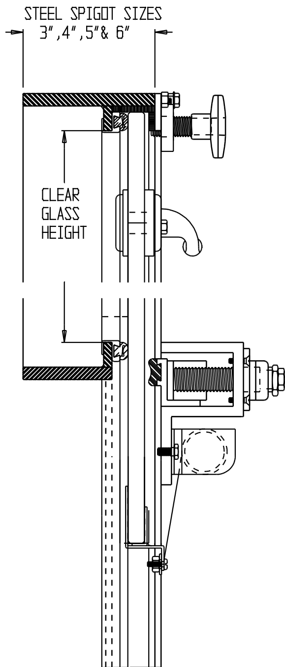
VERTICAL CROSS SECTION
